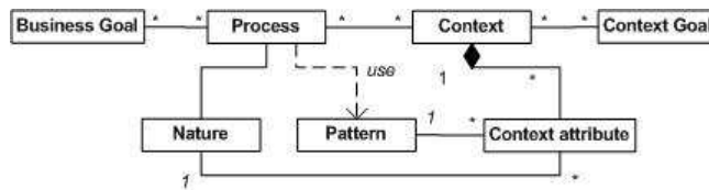
Fig. 2. Meta-model of pattern adequacy evaluation
